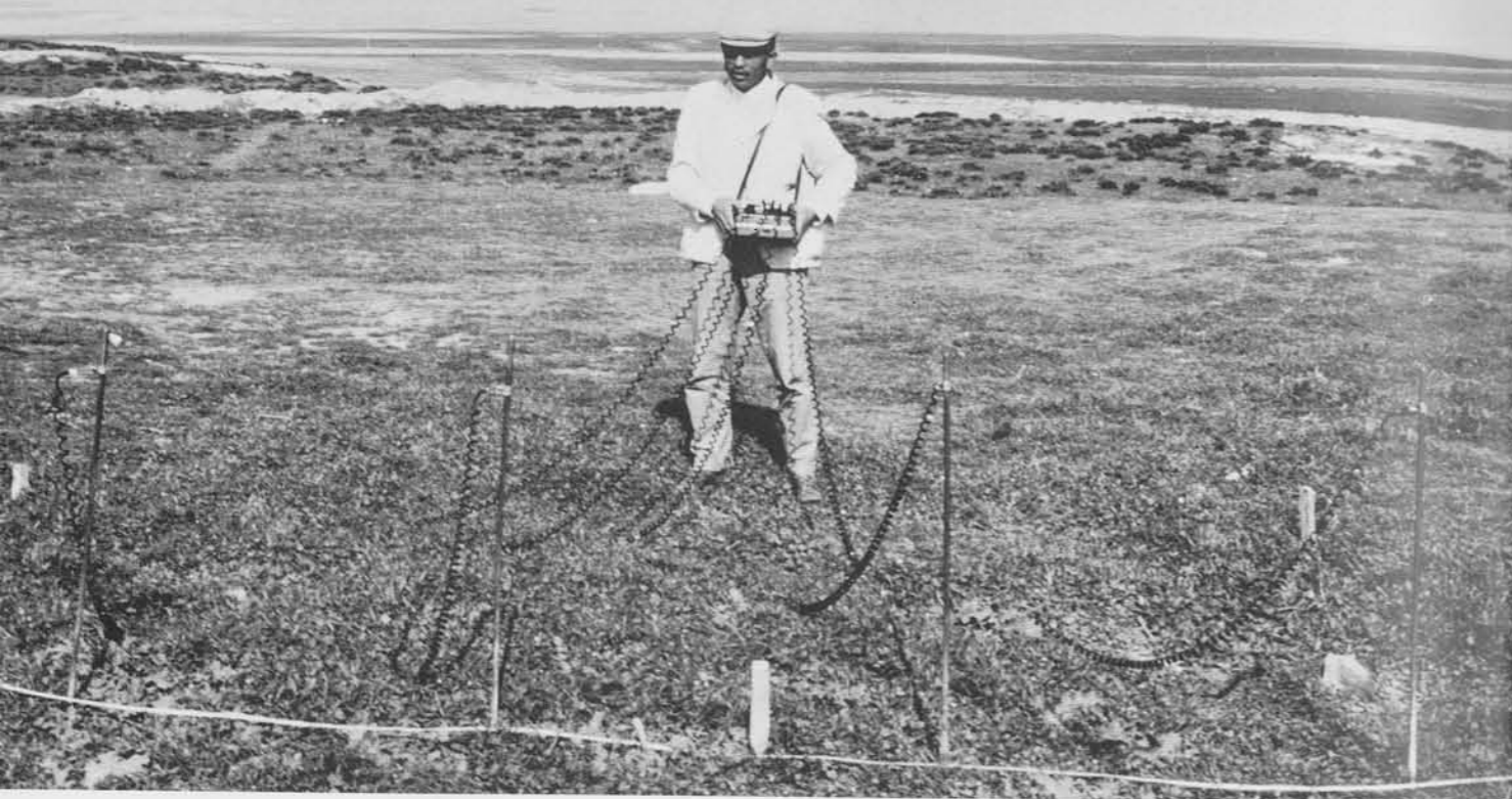
Geohm operated by Necmettin Bektöre at Gordion, Turkey. Four equally spaced rods are attached to Geohm with cables. Current is sent through outer two electrodes and the difference of potential (converted to resistivity units) is detected between the inner two.
