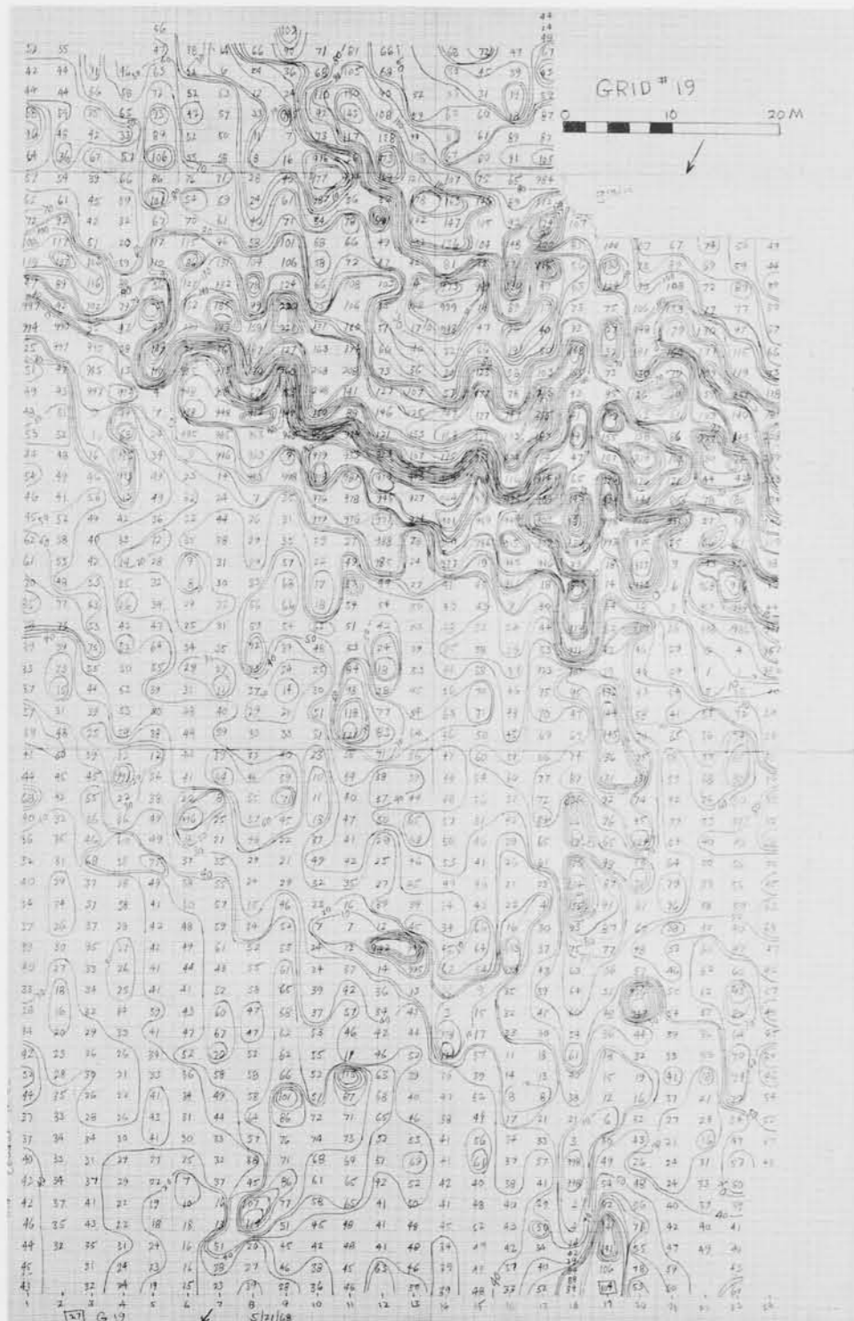
Cesium magnetometer Grid No. 19. Closely spaced contours in upper part probably represent rows of houses, Elis, Greece.
